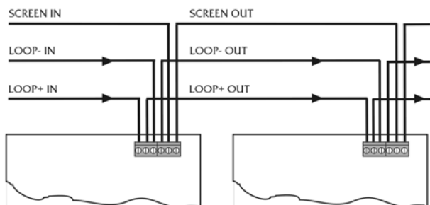
Fig 4 - Wiring Diagram (representation only)
